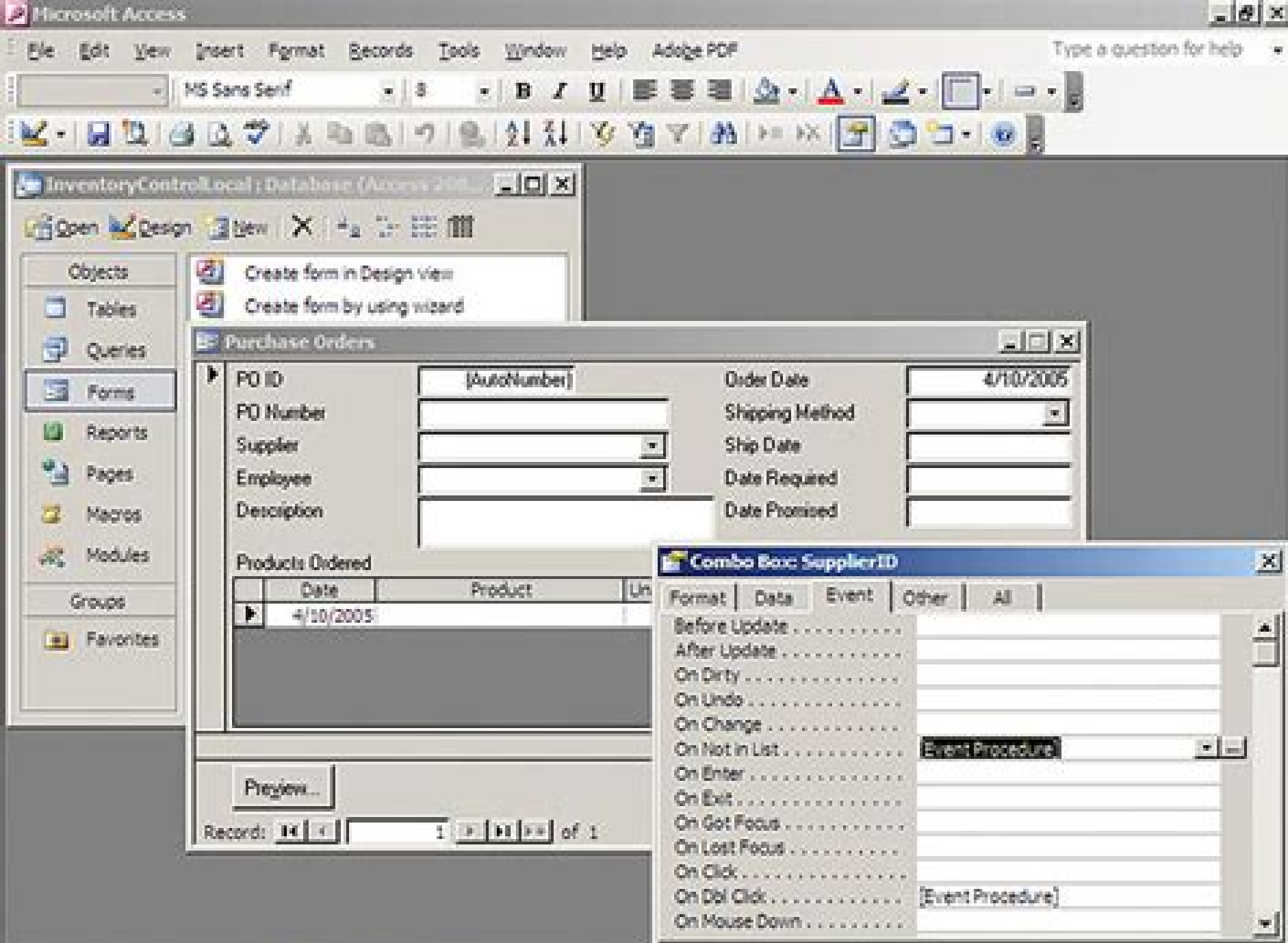
Macro or function that runs when combo box gets a Not In List message
