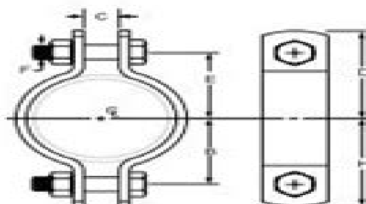
FIG. 212FP: LOADS (LBS) • WEIGHT (LBS) • DIMENSIONS (IN)
