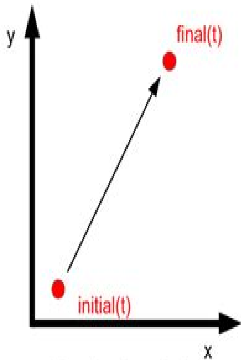
Classical particle
