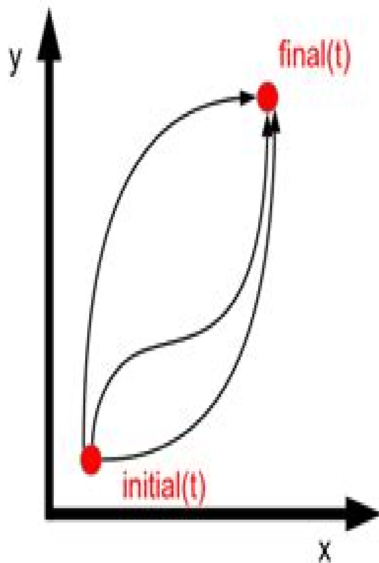
quantum particle
