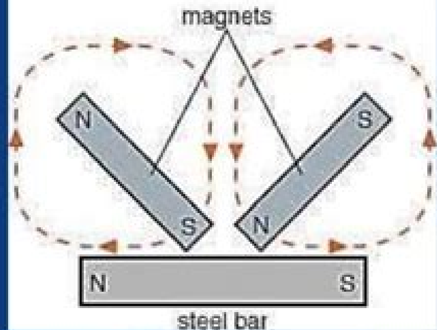
(b) Using two magnets
