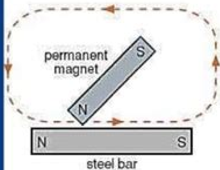
(a) Using one magnet
